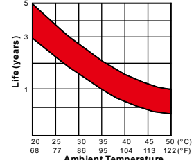
Influence of Temperature on Trickle(Float) Design Life
